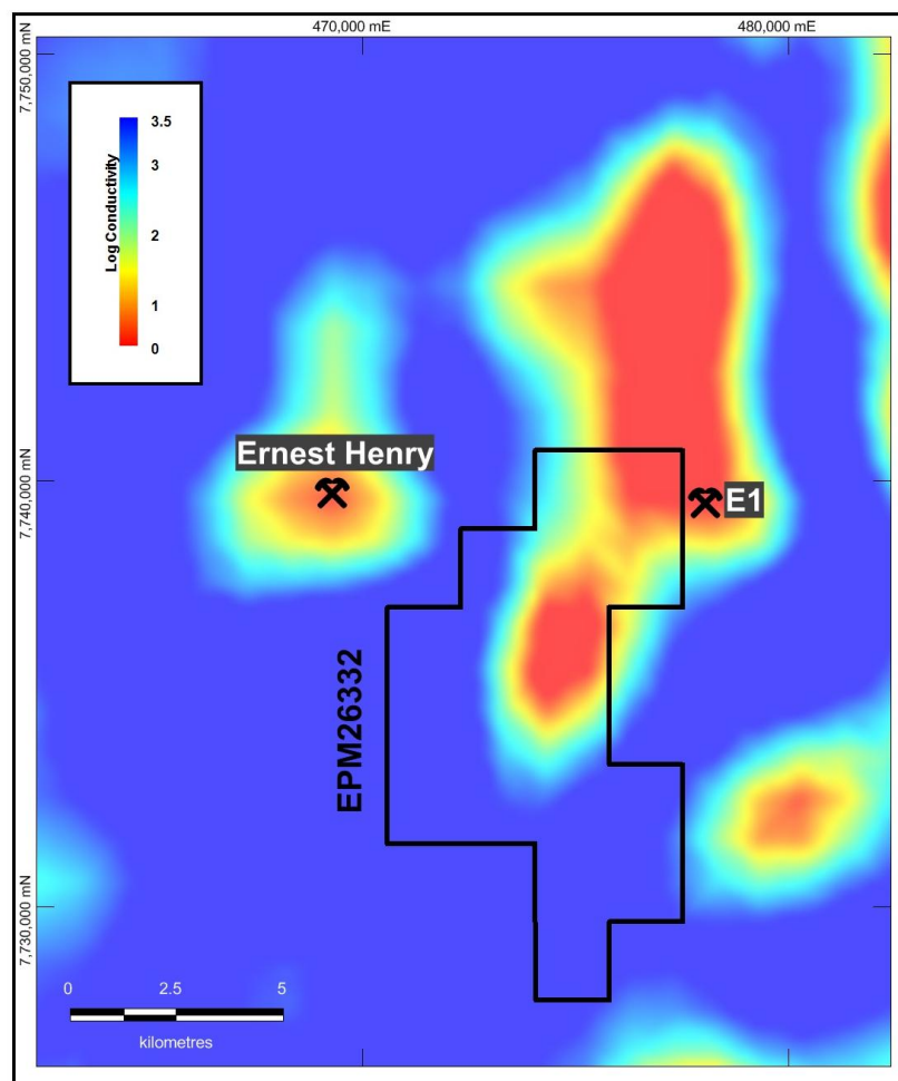
Figure 1: MT conductivity depth slice over EPM26332
