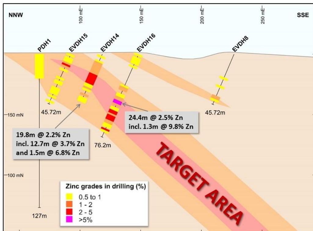
Figure 1: Cross section showing previous drilling and target area. Mineralisation is open at depth.
