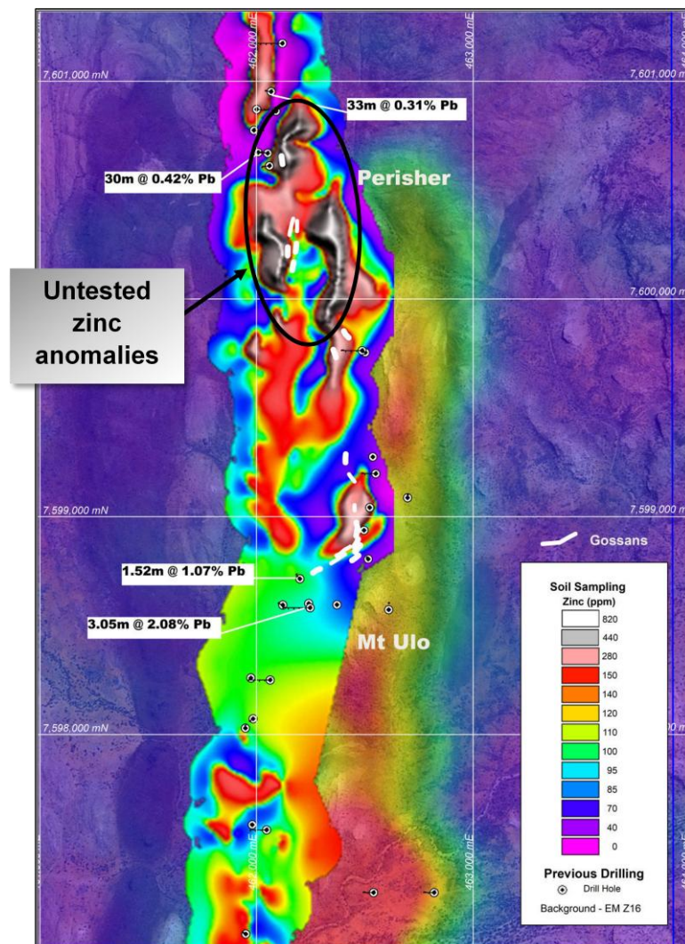
Figure 1: Zinc soil anomalies at Mt Ulo/Perisher, over airborne EM
